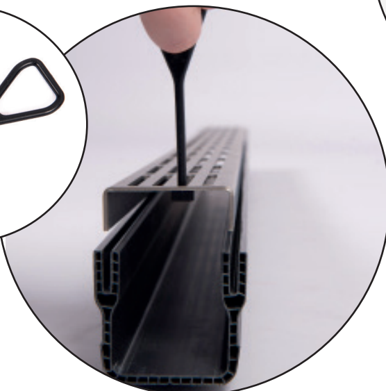
Lifting Tool
